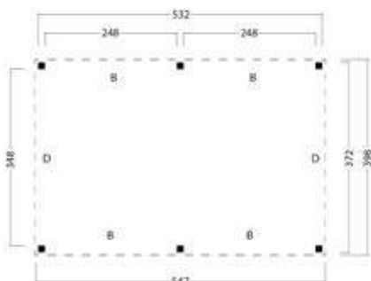
Basis
