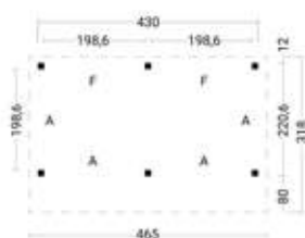
Basis L
