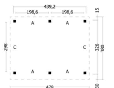
Basis L
