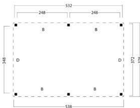
Basis
