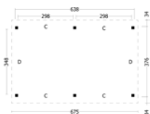
Basis XL
