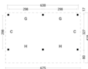
Basis XL
